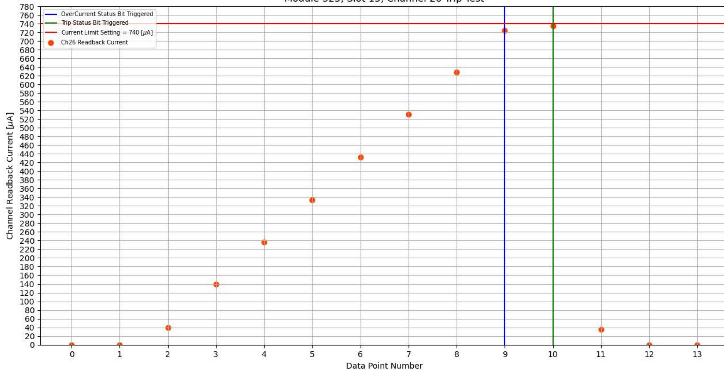
Module 325, Slot 15, Channel 26 Trip Test
