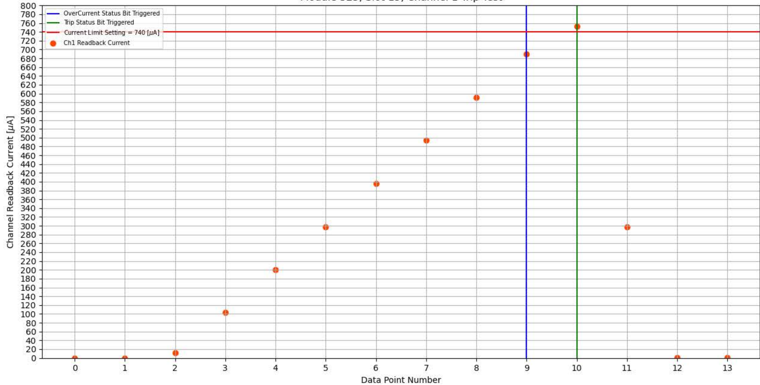
Module 325, Slot 15, Channel 1 Trip Test
