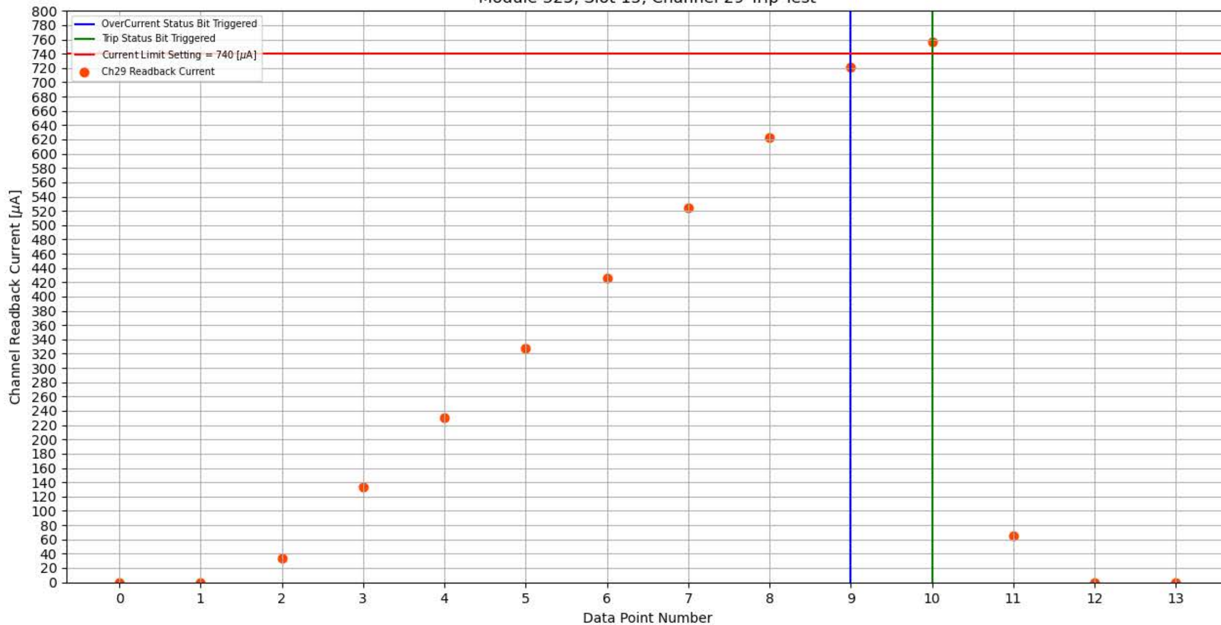
Module 325, Slot 15, Channel 29 Trip Test
