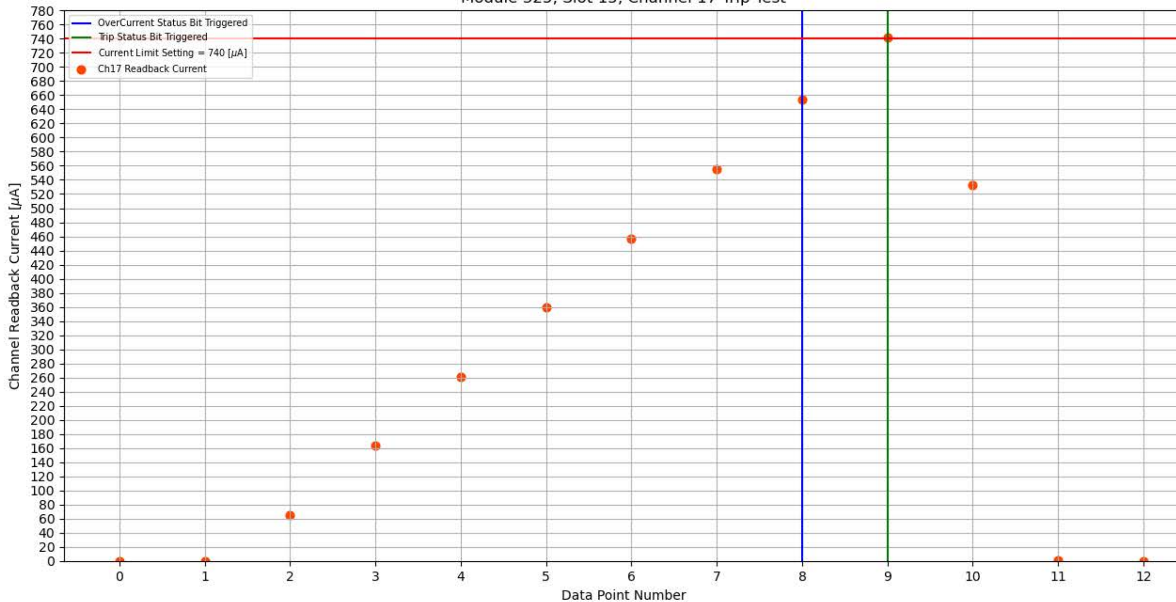
Module 325, Slot 15, Channel 17 Trip Test
