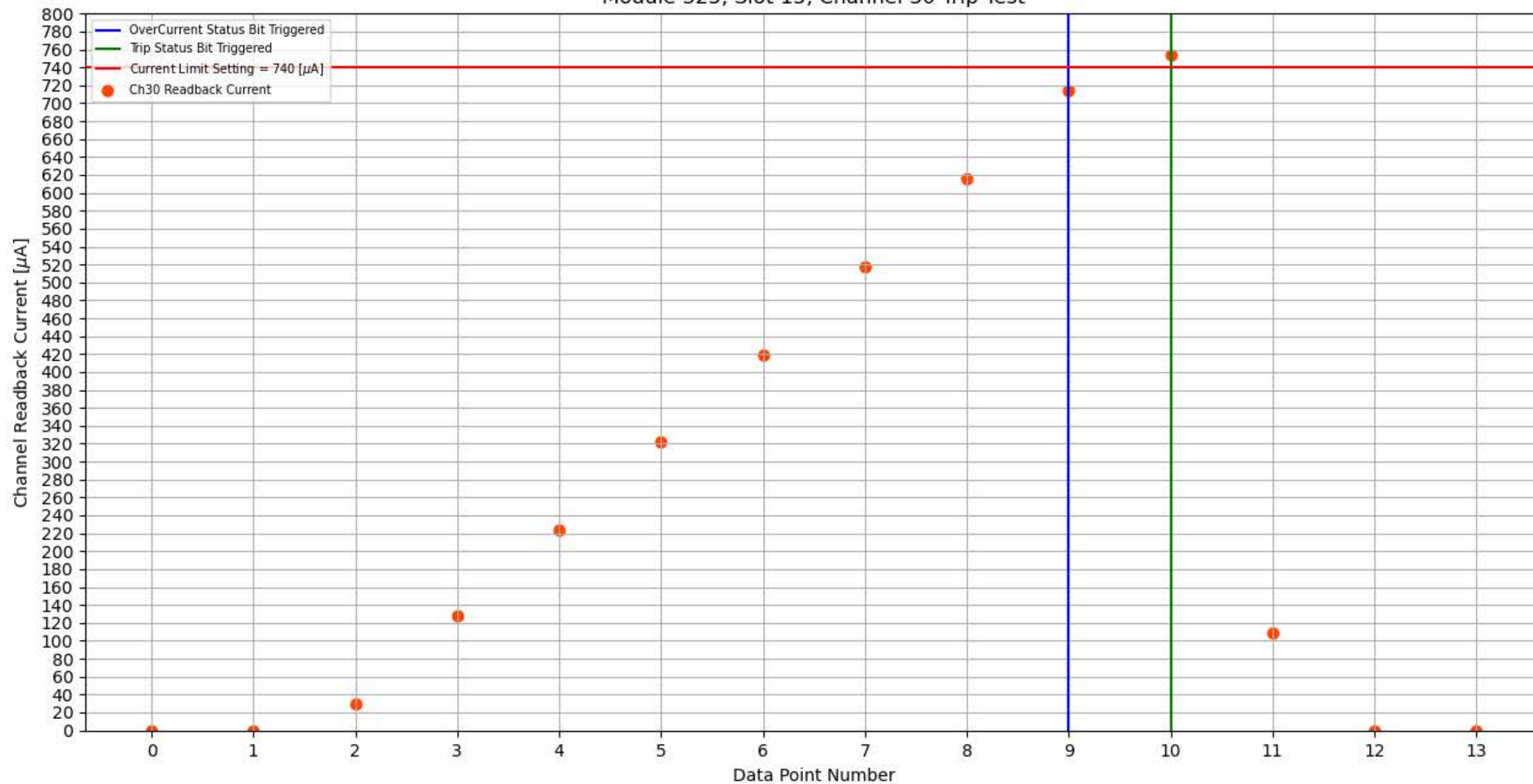
Module 325, Slot 15, Channel 30 Trip Test
