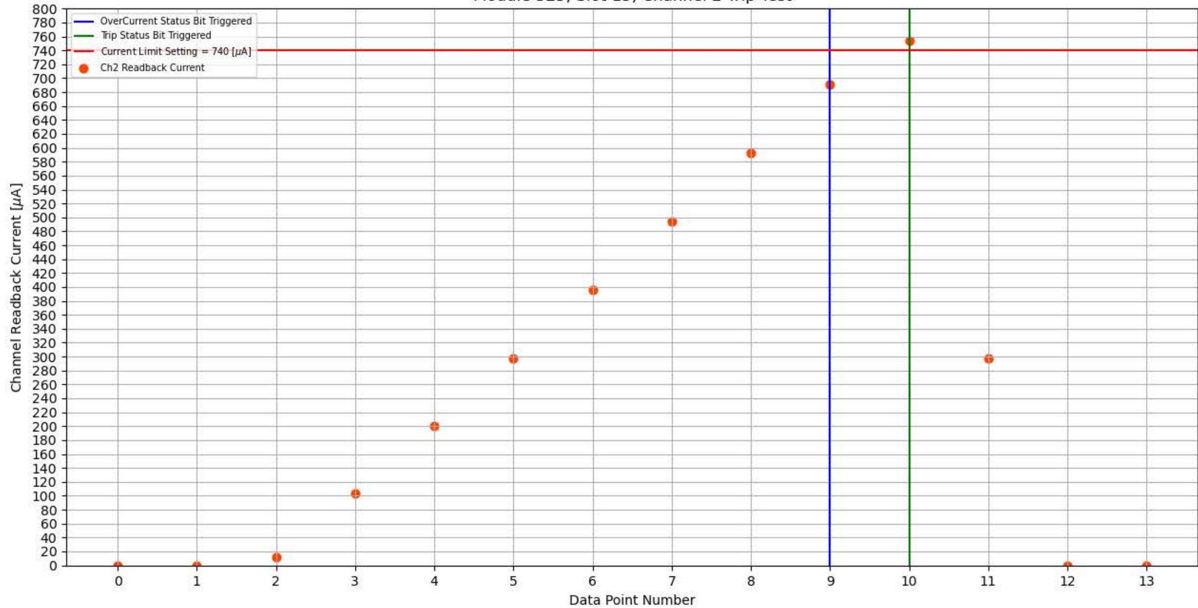
Module 325, Slot 15, Channel 2 Trip Test
