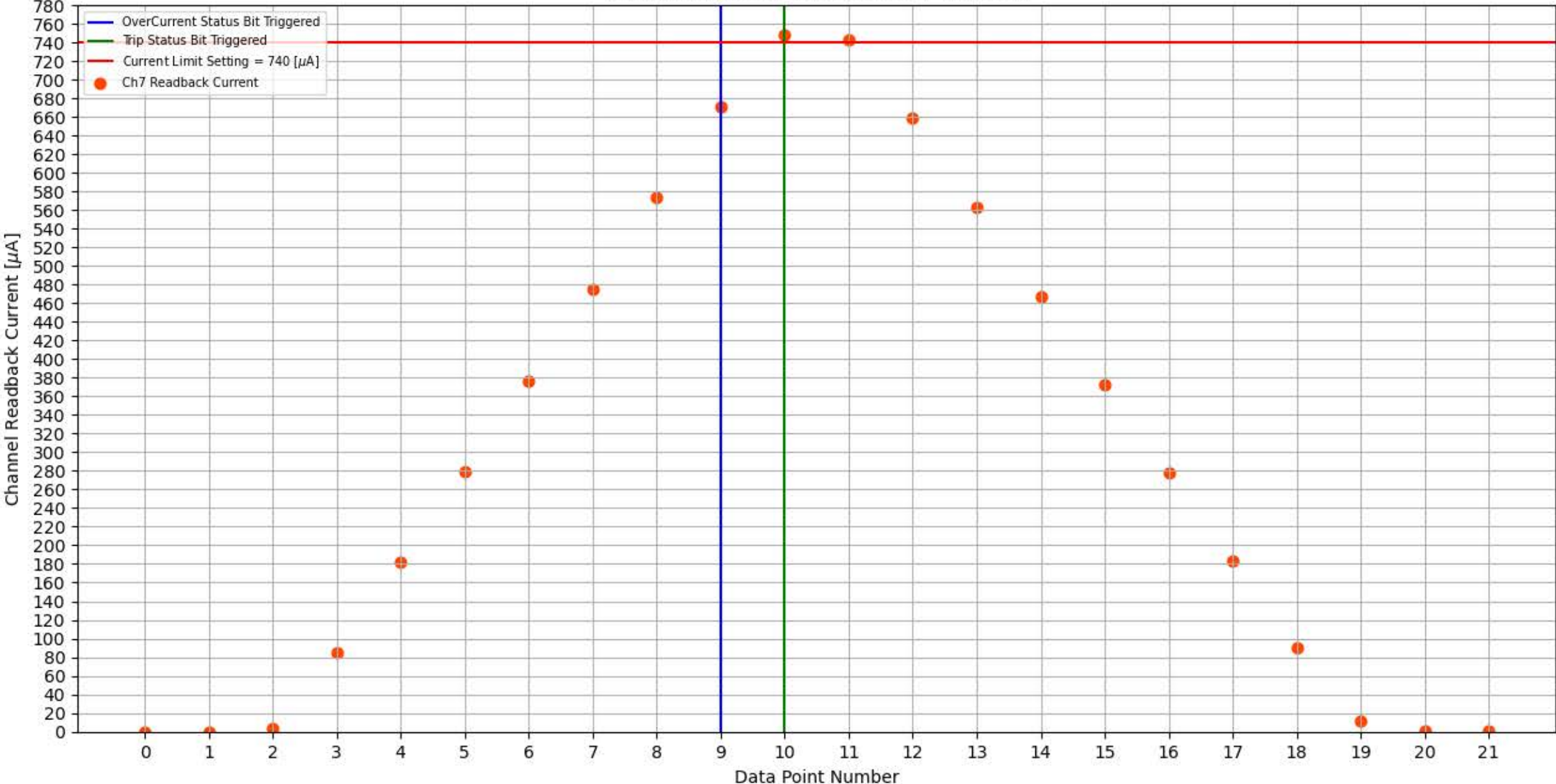
Module 325, Slot 15, Channel 7 Trip Test
