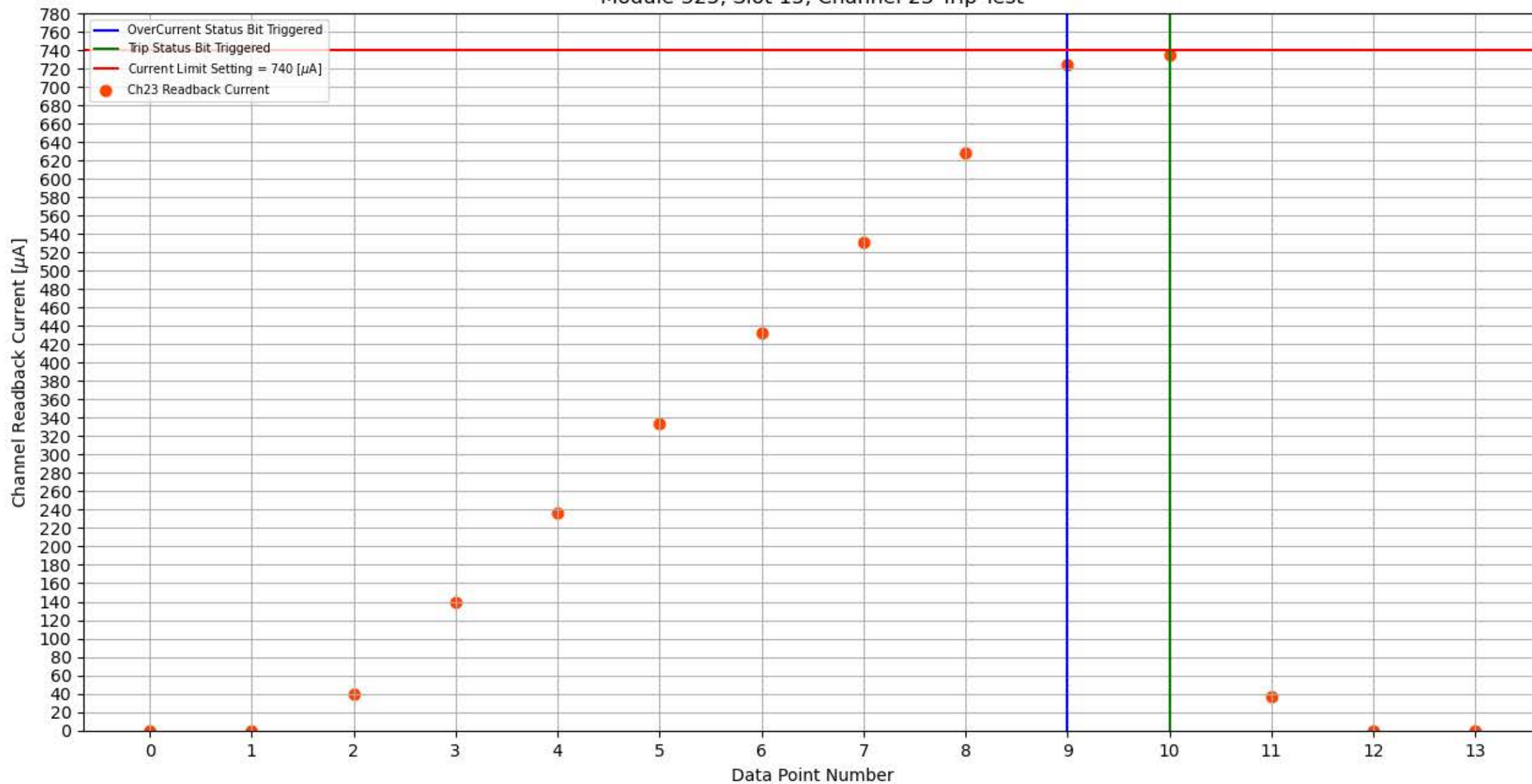
Module 325, Slot 15, Channel 23 Trip Test
