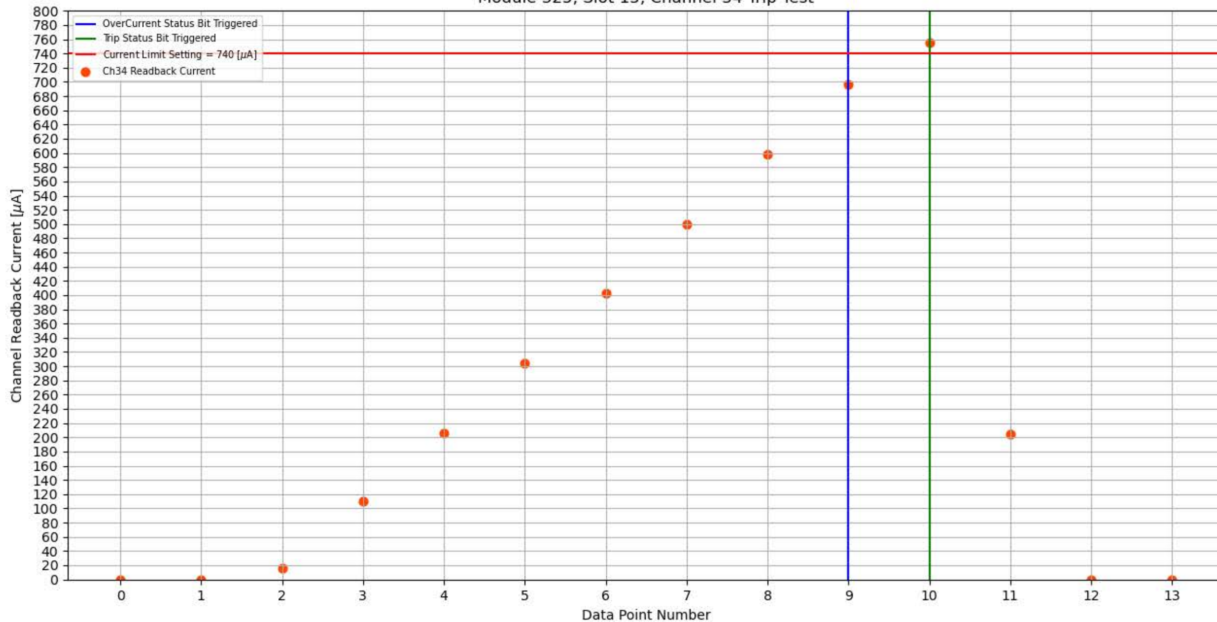
Module 325, Slot 15, Channel 34 Trip Test
