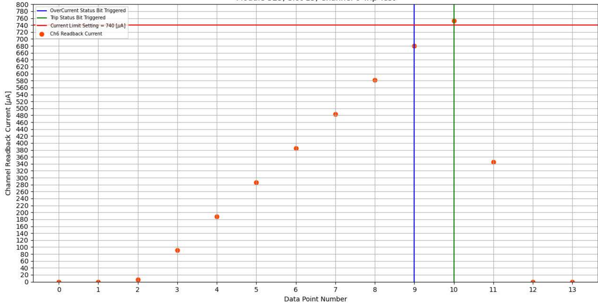
Module 325, Slot 15, Channel 6 Trip Test
