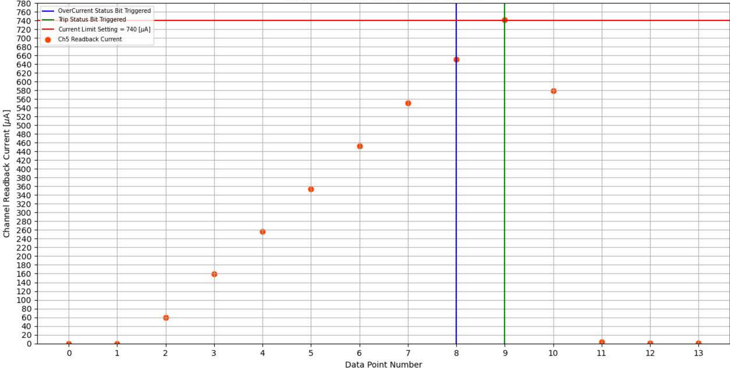
Module 325, Slot 15, Channel 5 Trip Test
