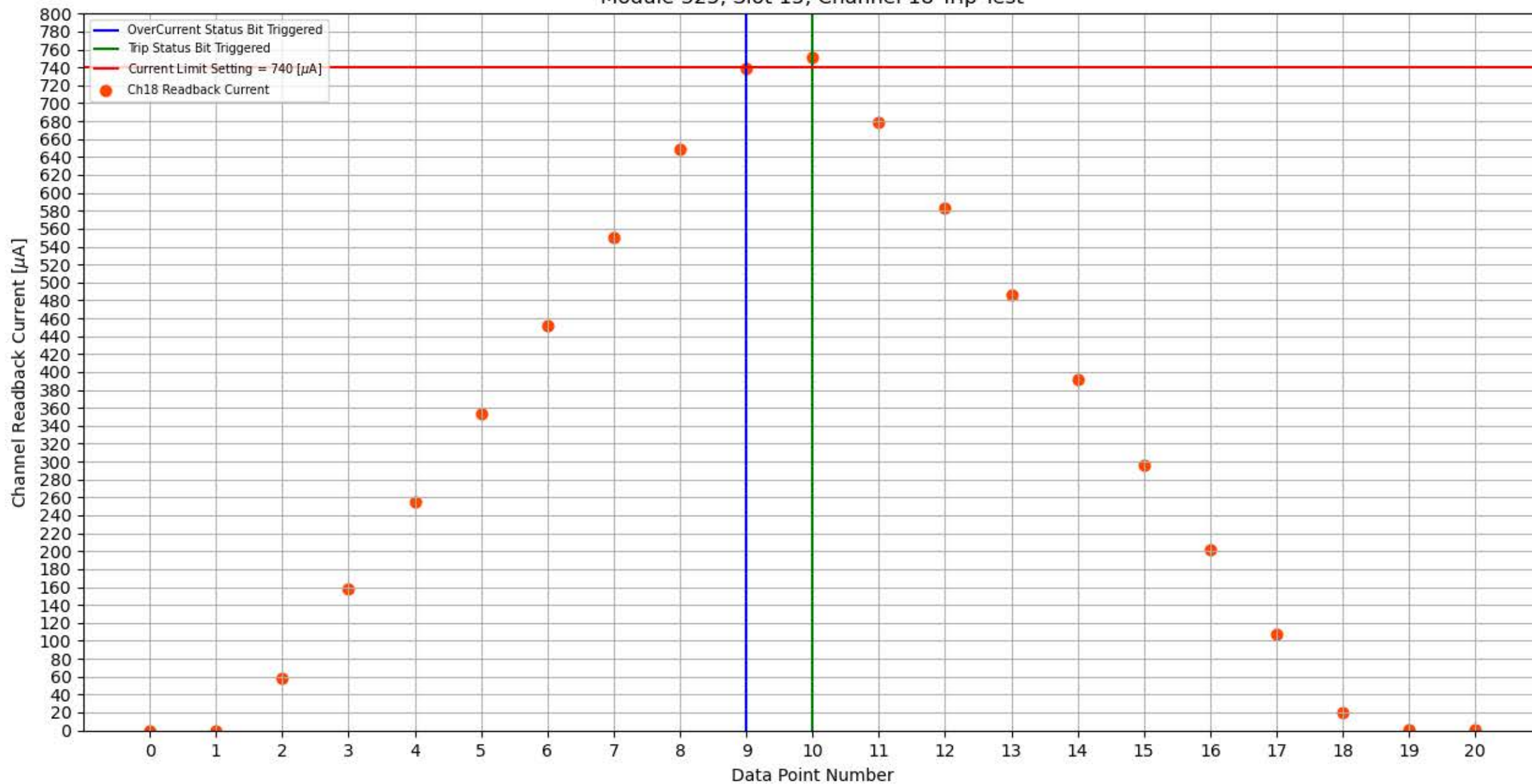
Module 325, Slot 15, Channel 18 Trip Test
