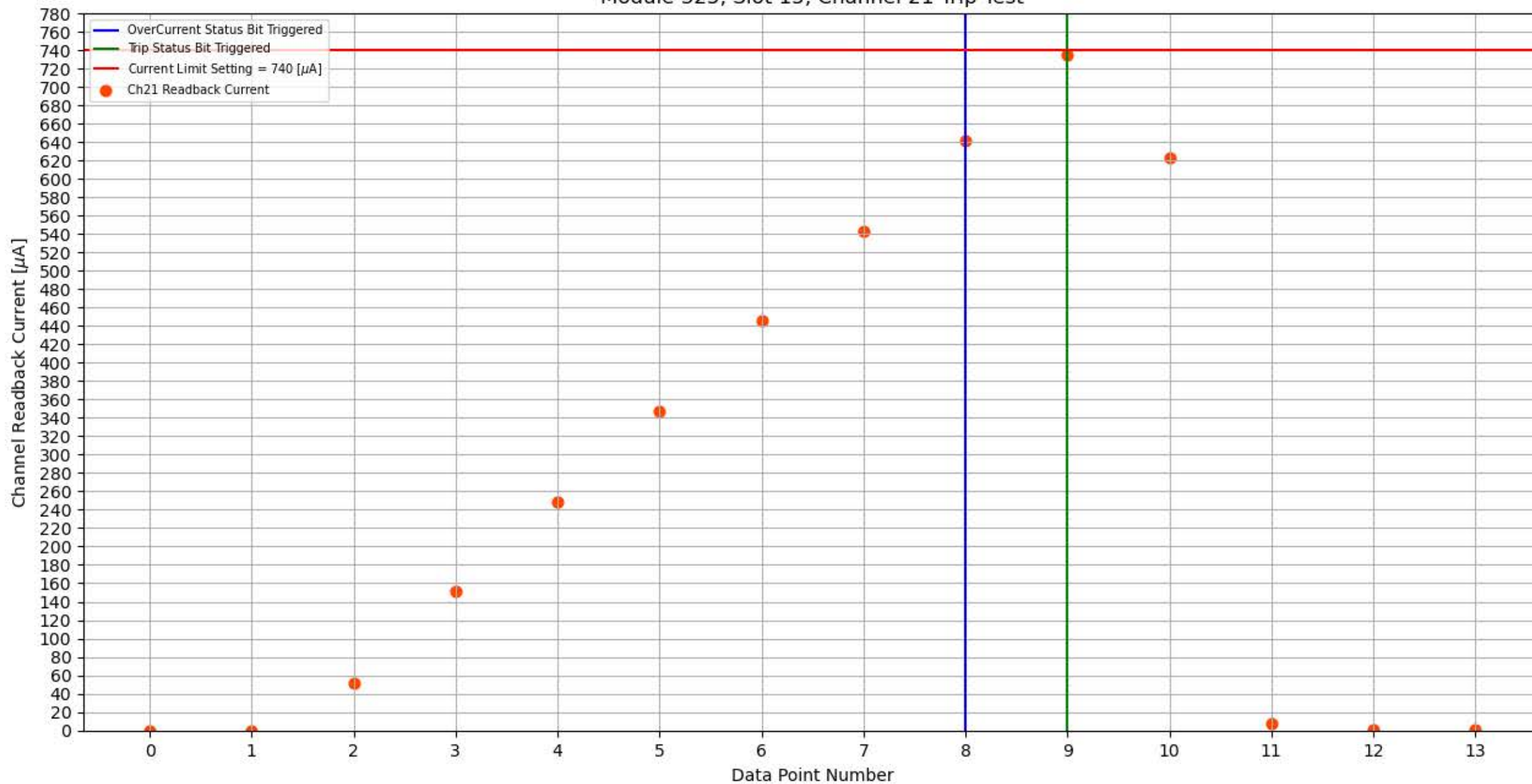
Module 325, Slot 15, Channel 21 Trip Test
