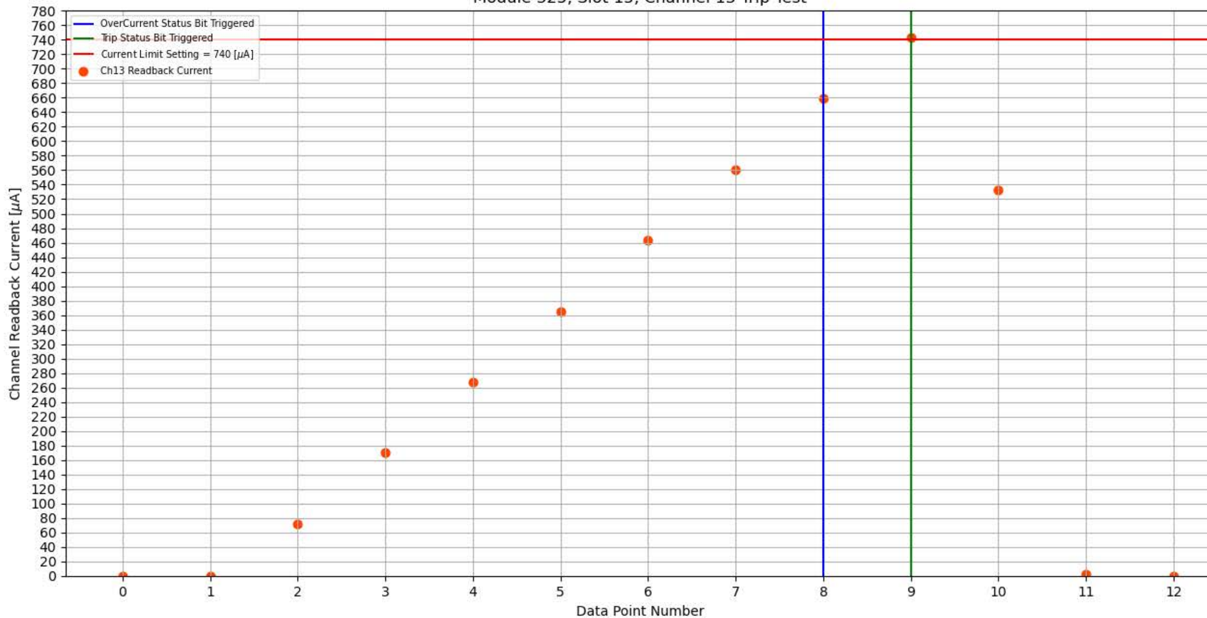
Module 325, Slot 15, Channel 13 Trip Test
