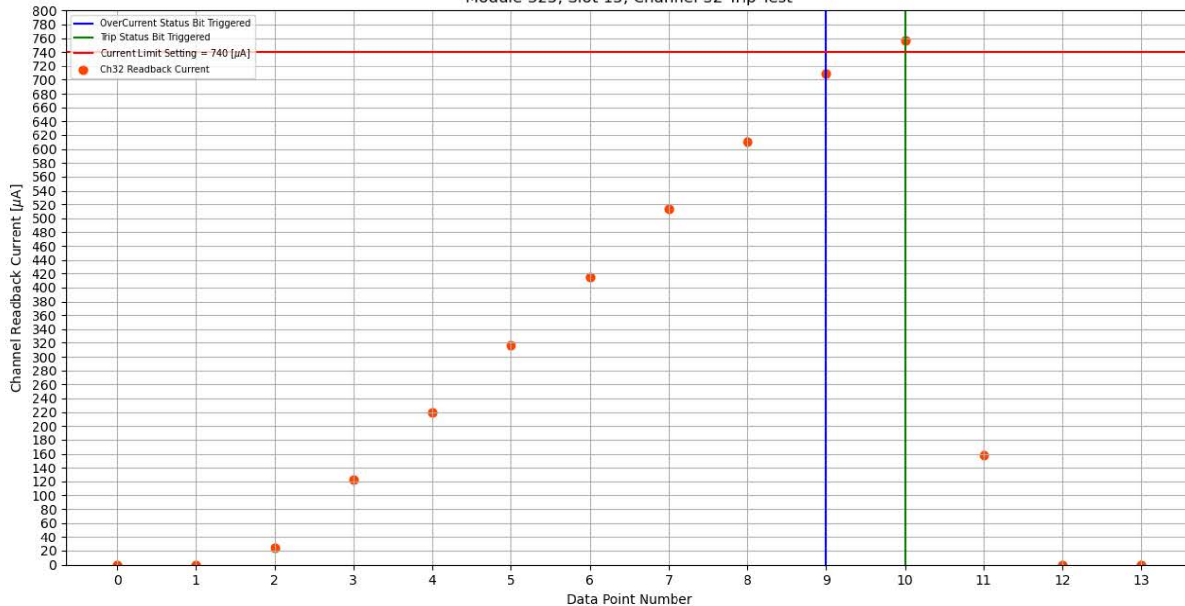
Module 325, Slot 15, Channel 32 Trip Test
