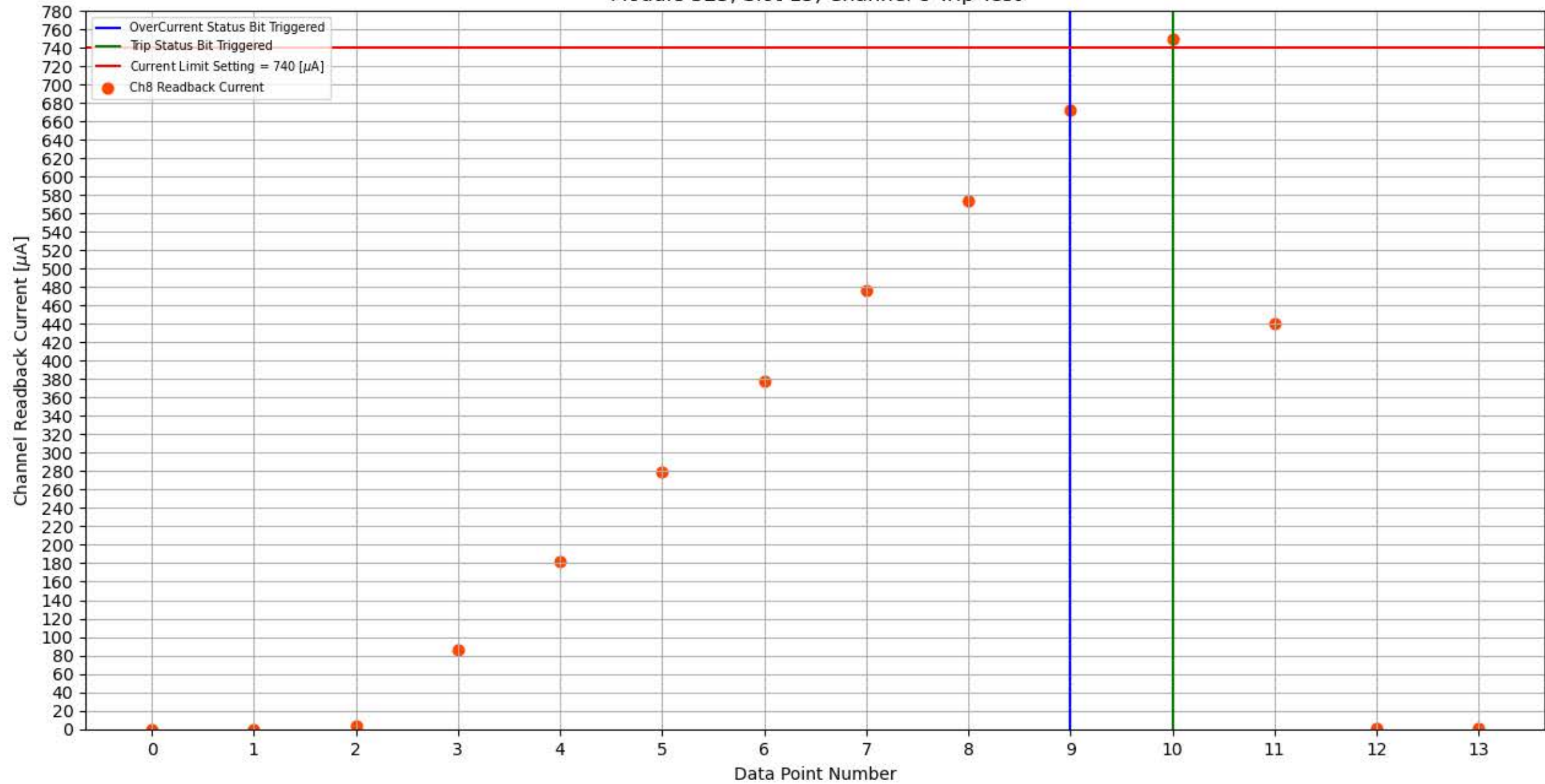
Module 325, Slot 15, Channel 8 Trip Test
