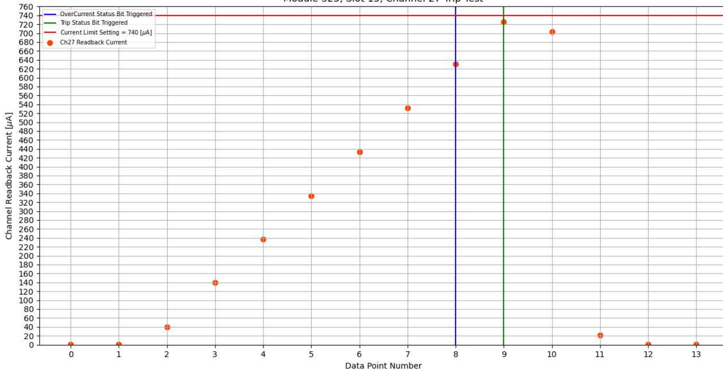
Module 325, Slot 15, Channel 27 Trip Test
