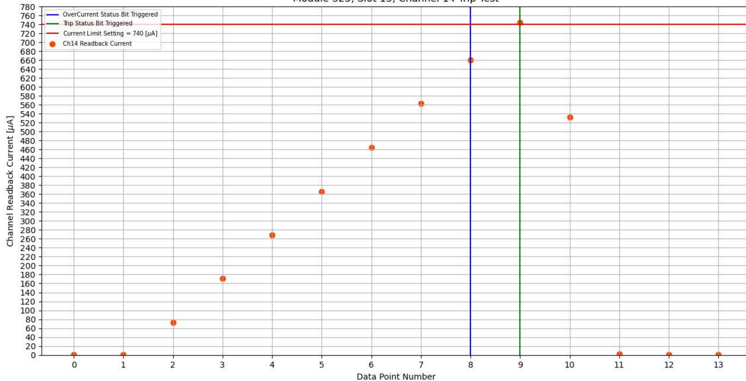
Module 325, Slot 15, Channel 14 Trip Test
