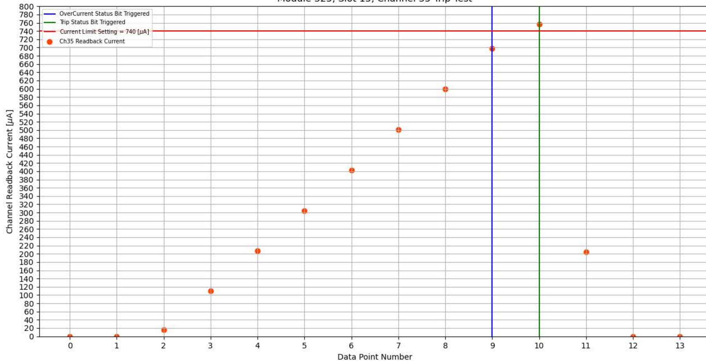
Module 325, Slot 15, Channel 35 Trip Test
