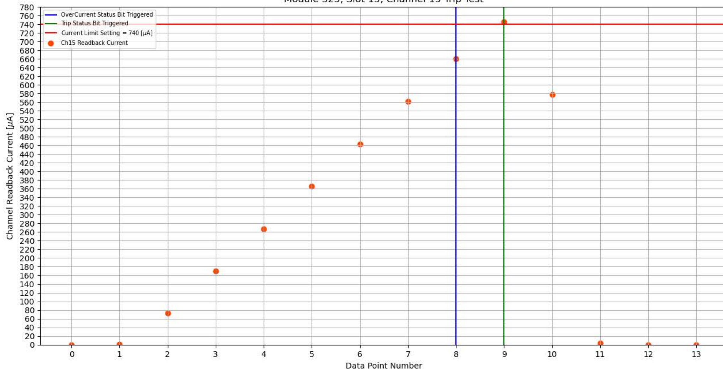
Module 325, Slot 15, Channel 15 Trip Test
