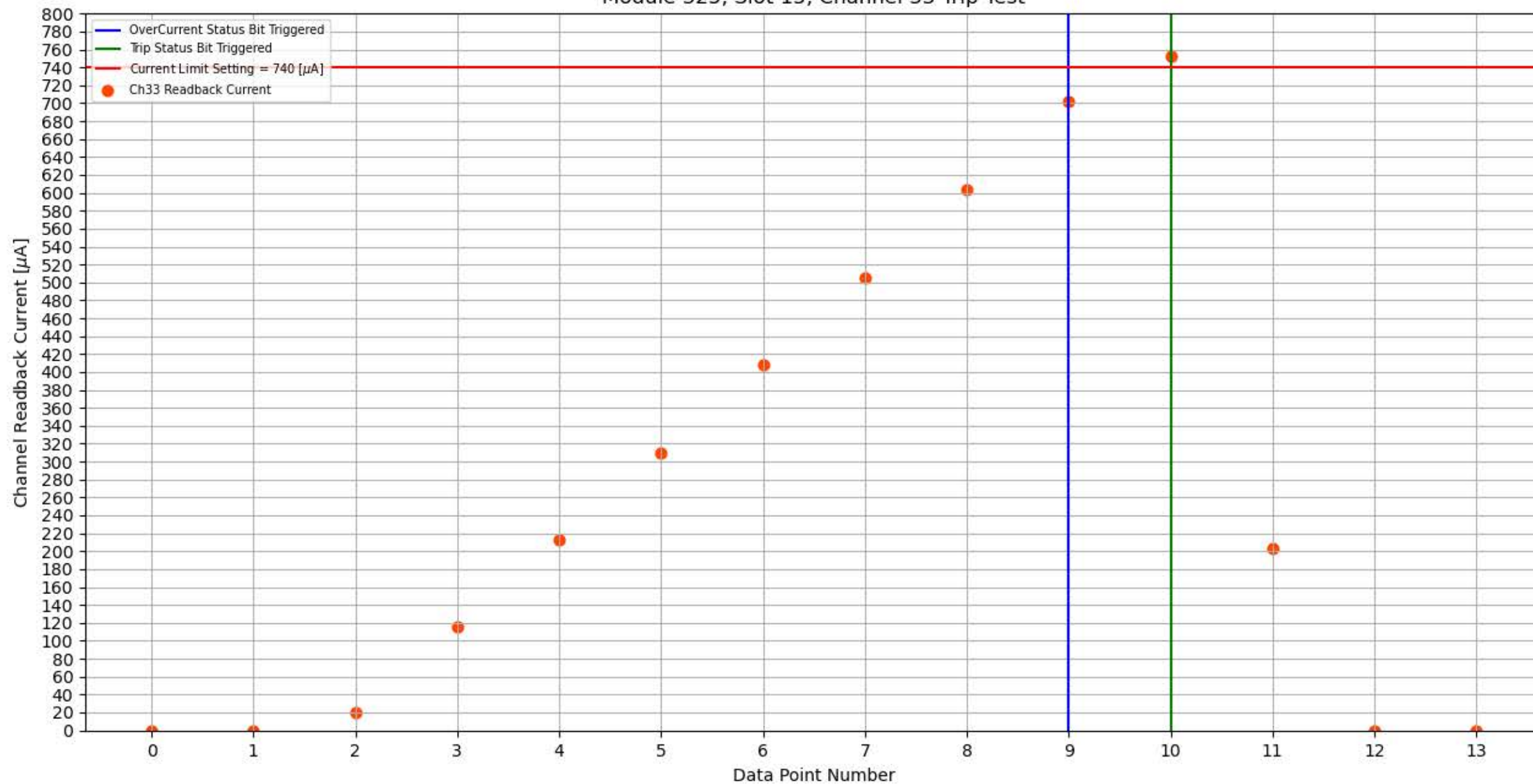
Module 325, Slot 15, Channel 33 Trip Test
