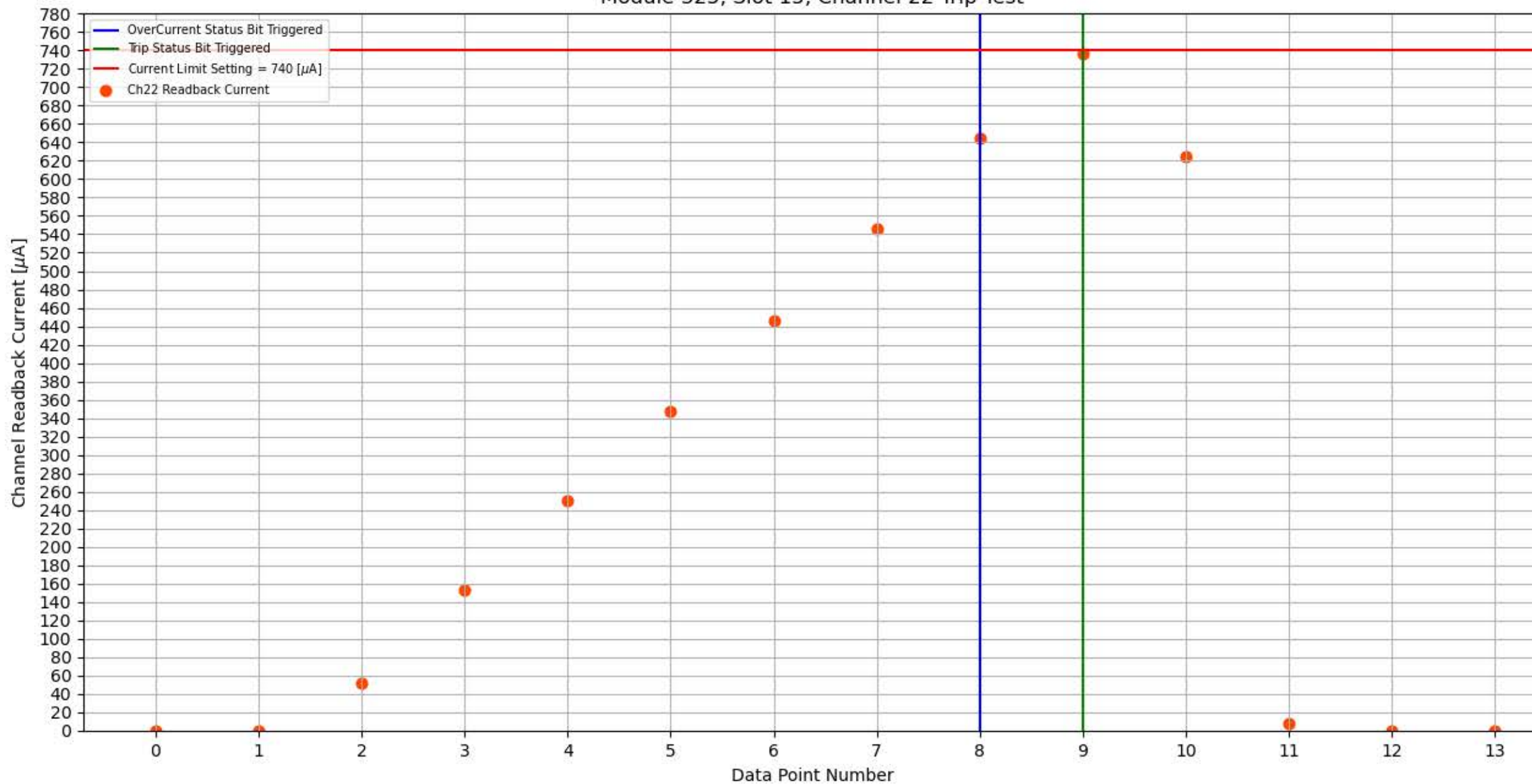
Module 325, Slot 15, Channel 22 Trip Test
