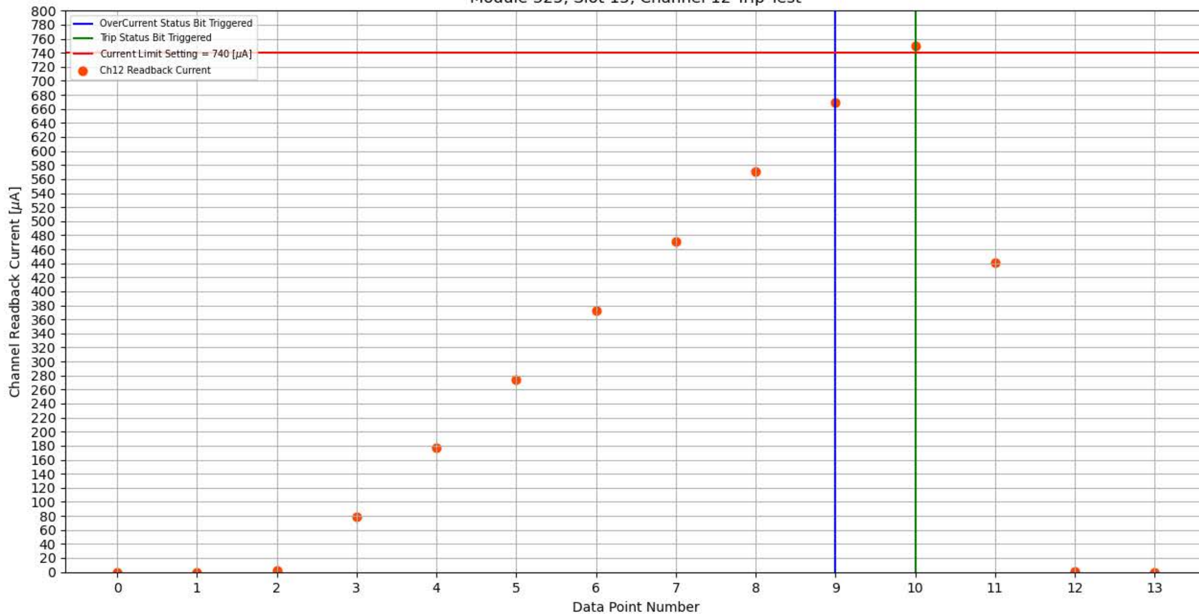
Module 325, Slot 15, Channel 12 Trip Test
