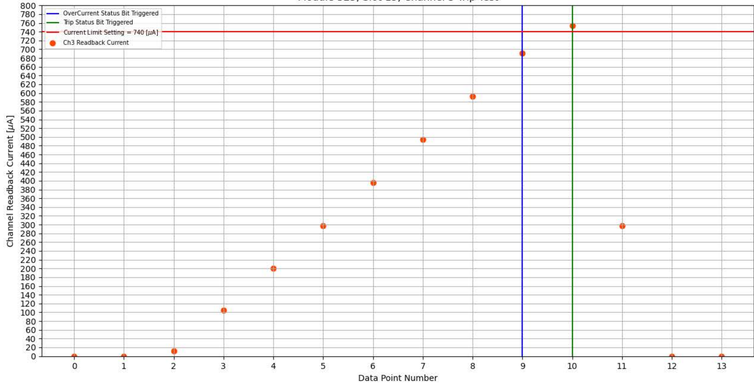
Module 325, Slot 15, Channel 3 Trip Test
