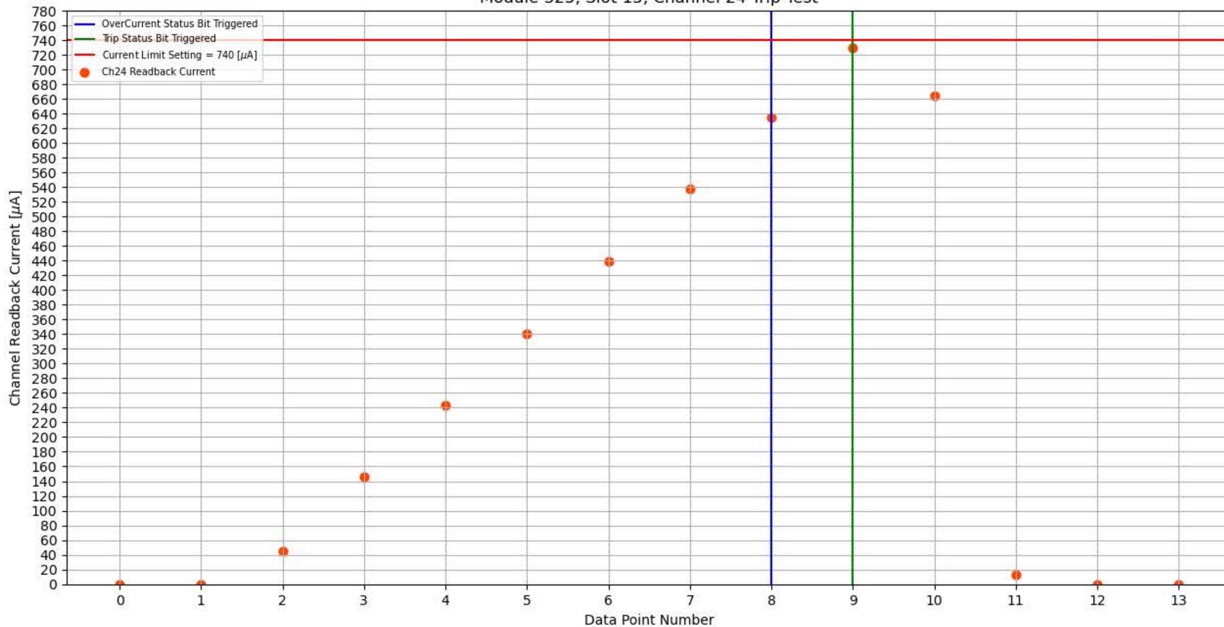
Module 325, Slot 15, Channel 24 Trip Test
