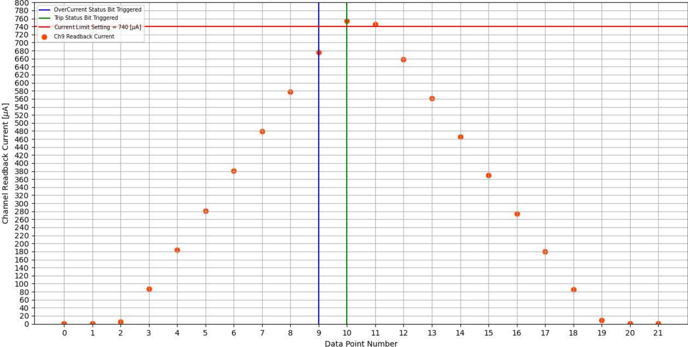
Module 325, Slot 15, Channel 9 Trip Test
