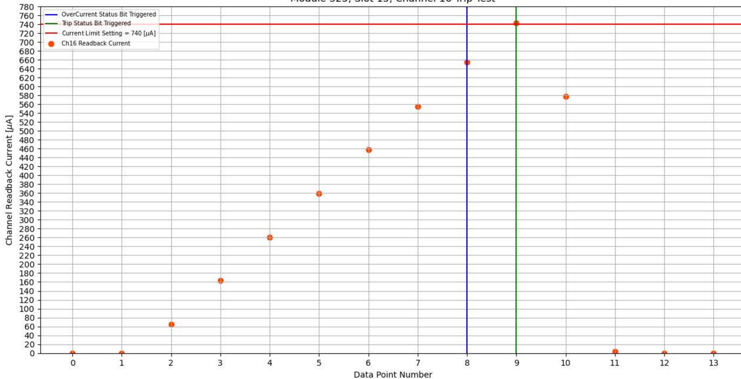
Module 325, Slot 15, Channel 16 Trip Test
