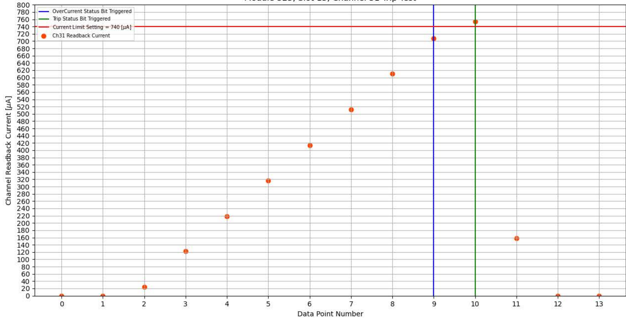
Module 325, Slot 15, Channel 31 Trip Test
