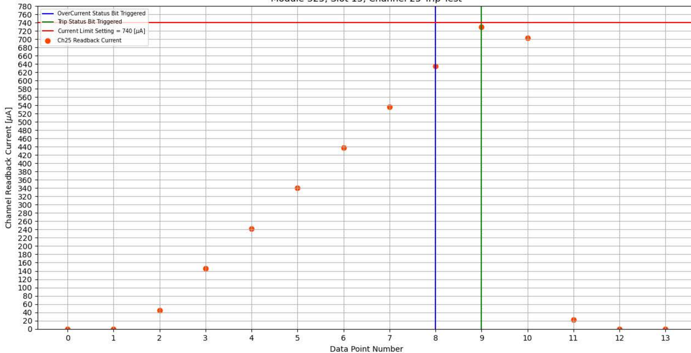
Module 325, Slot 15, Channel 25 Trip Test
