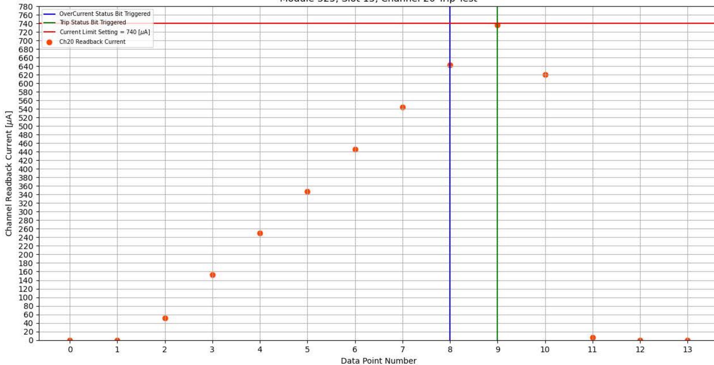
Module 325, Slot 15, Channel 20 Trip Test
