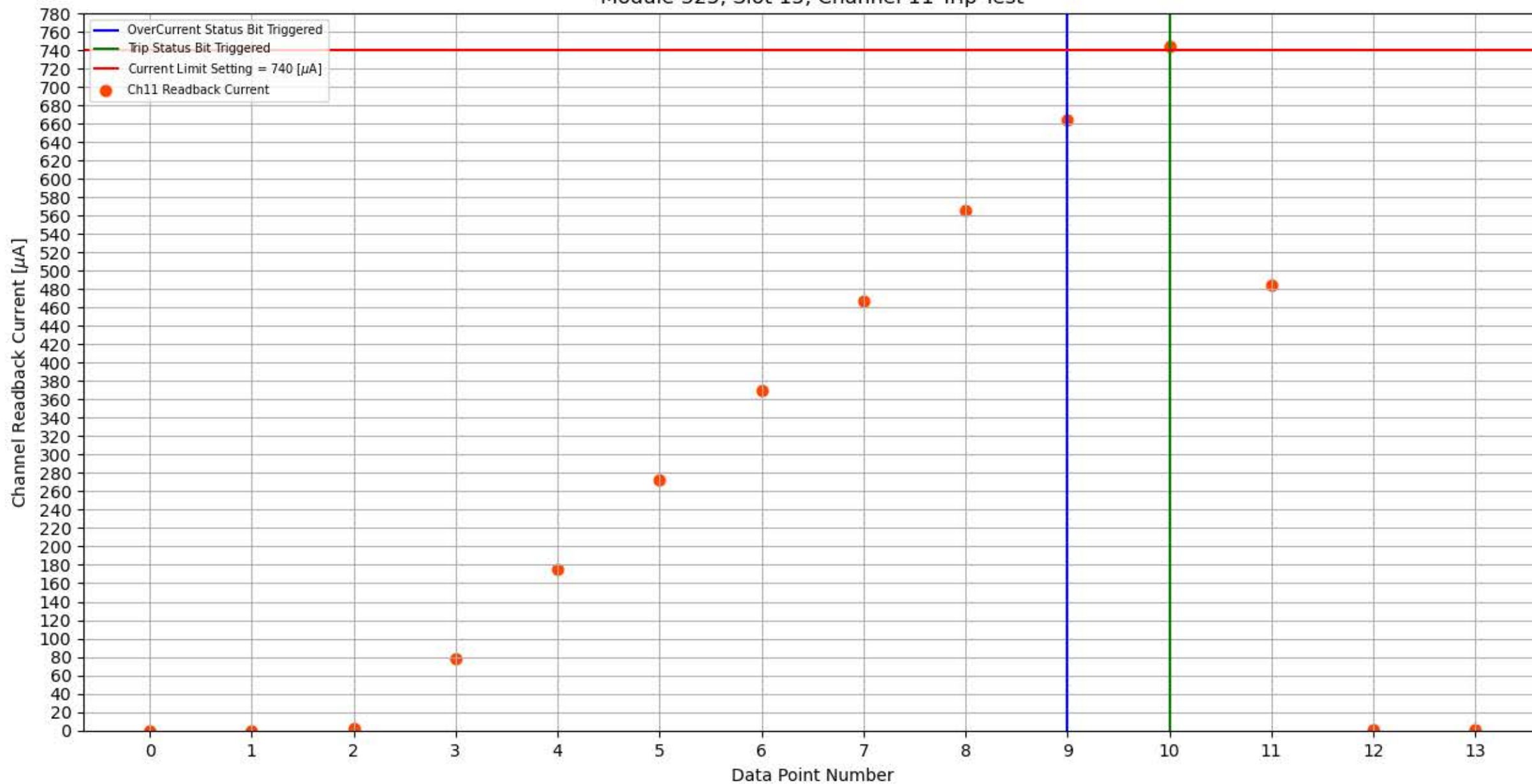
Module 325, Slot 15, Channel 11 Trip Test
