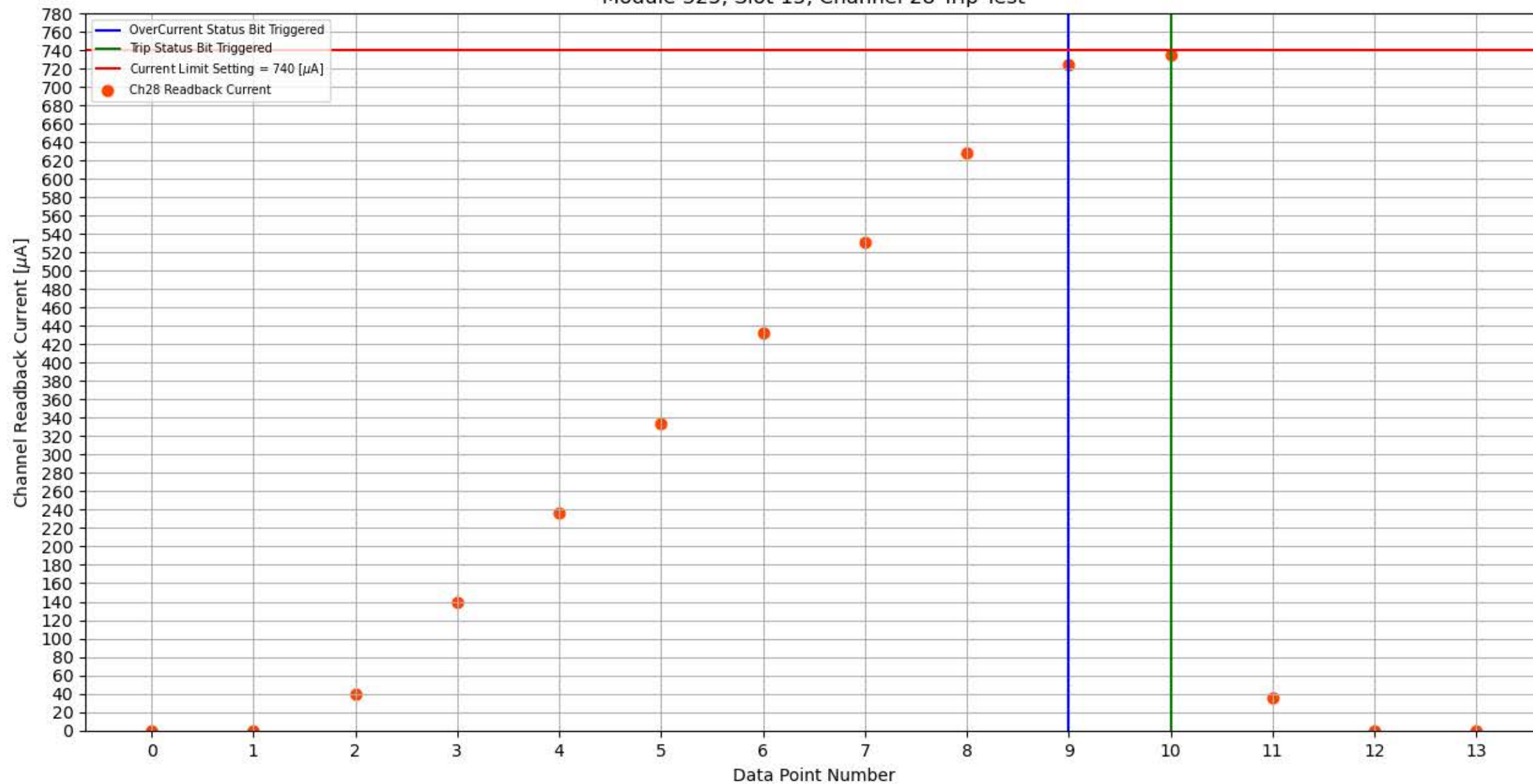
Module 325, Slot 15, Channel 28 Trip Test
