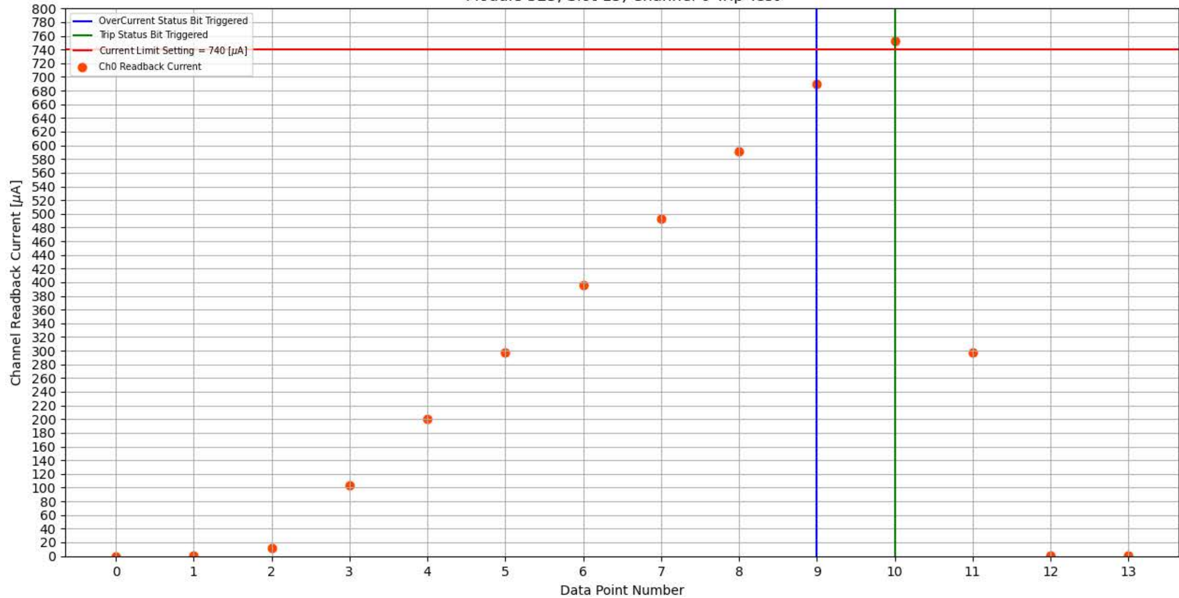
Module 325, Slot 15, Channel 0 Trip Test
