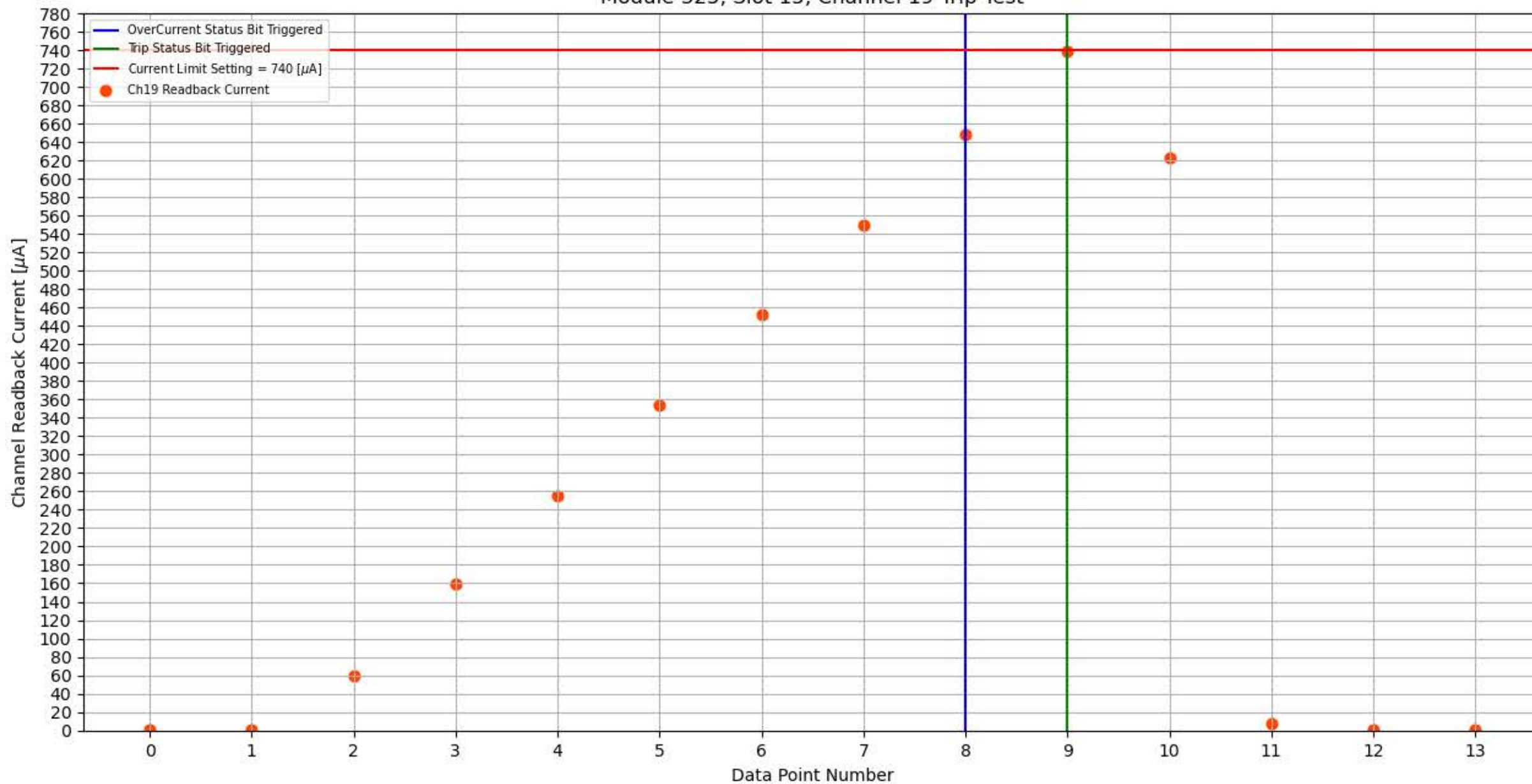
Module 325, Slot 15, Channel 19 Trip Test
