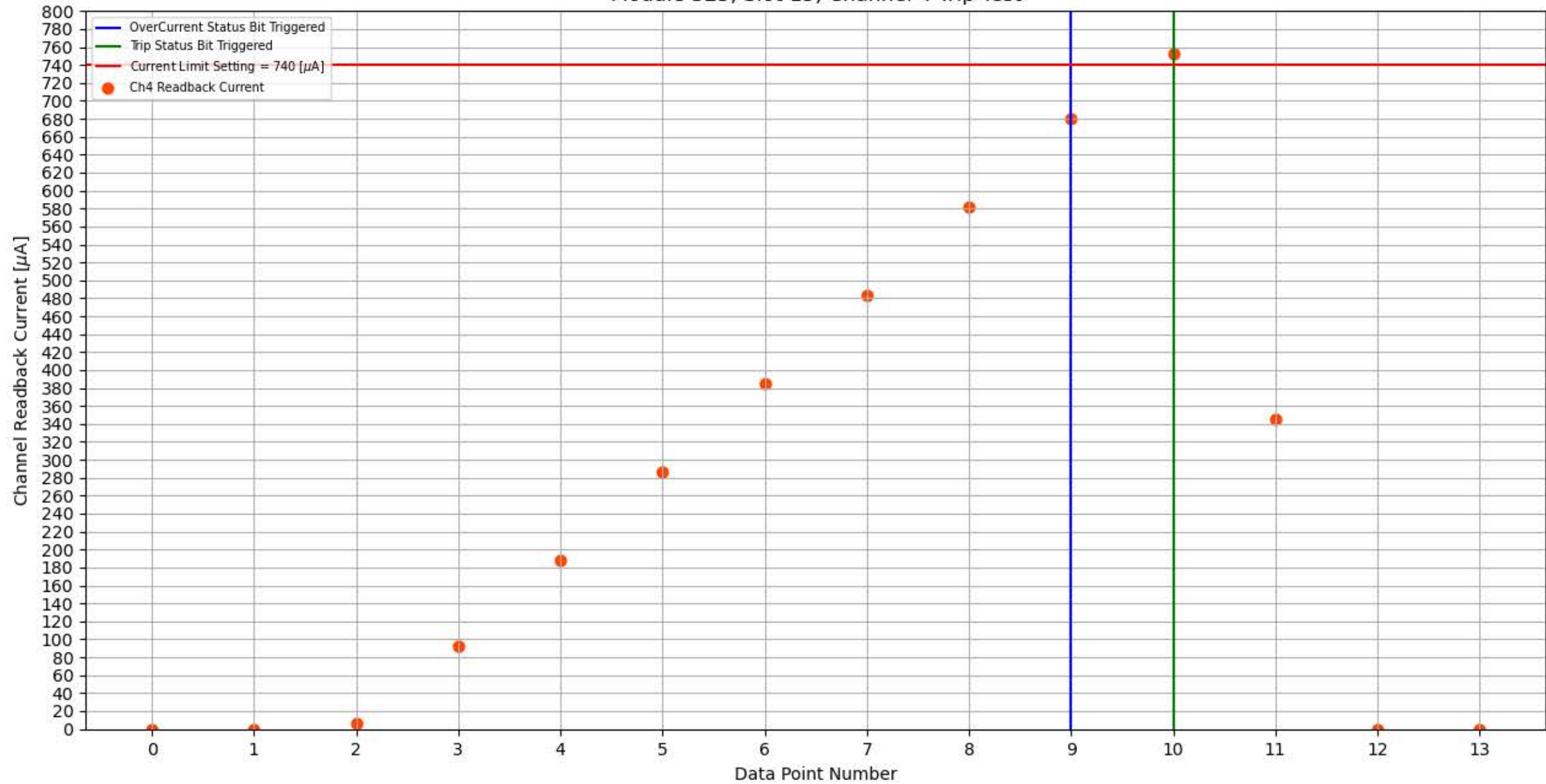
Module 325, Slot 15, Channel 4 Trip Test
